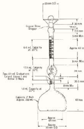
FIG. 1 Le Chatelier Flask for Density Test
